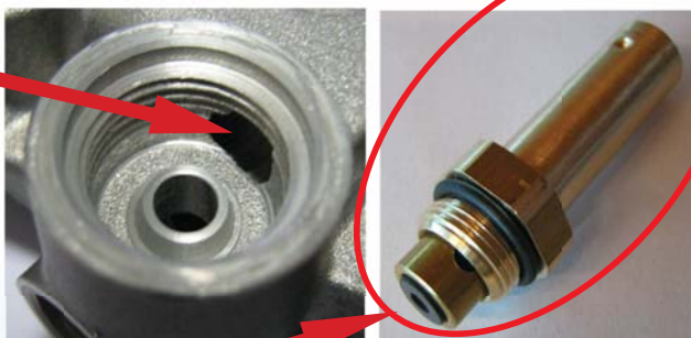
Fig.3/4 - Alaska Super solenoid internal passage and solenoid core
