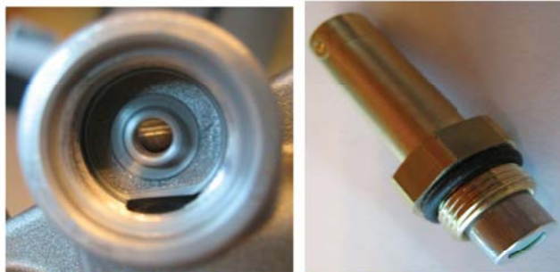
Fig.1/2 - Alaska standard solenoid internal passage and solenoid core
